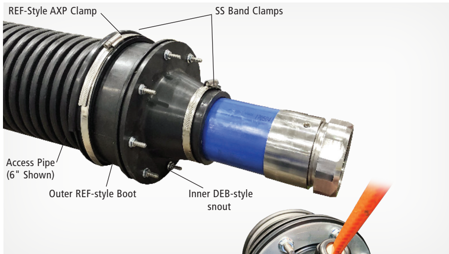
HEF-4020G Entry Fitting with Heat Tracing
